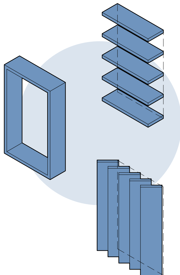
Figure 6: Solar Shading | Use solar shading devices to minimize unwanted solar heat gain.
