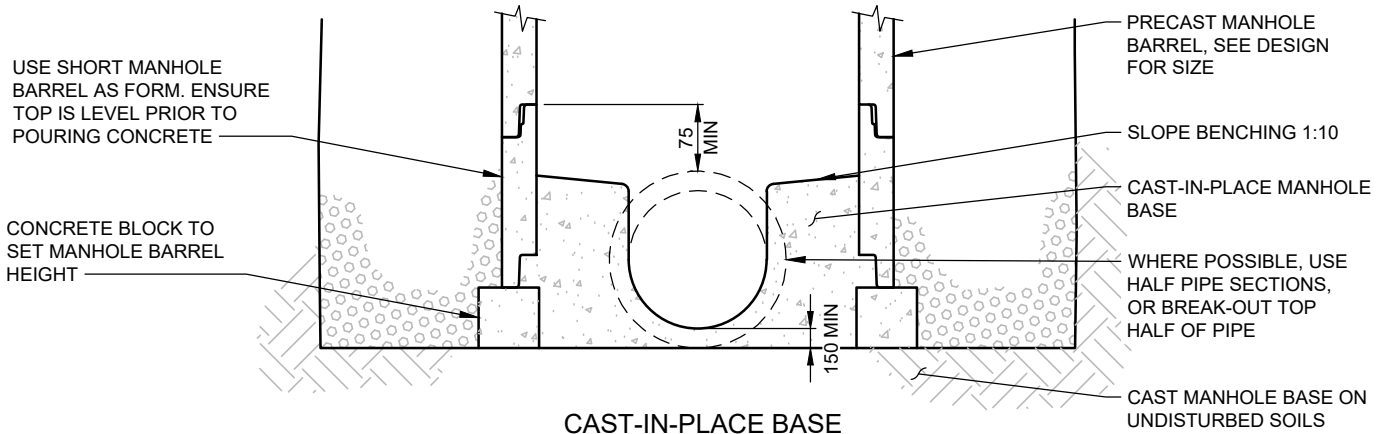
CAST-IN-PLACE BASE
