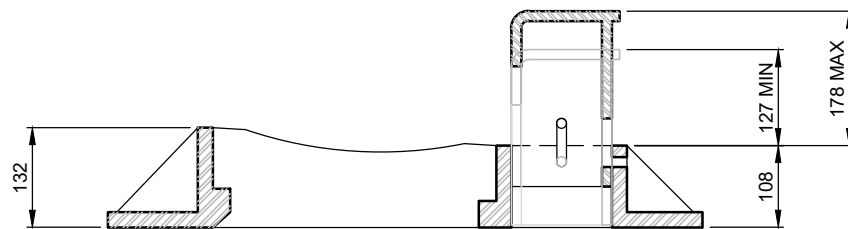
SECTION
