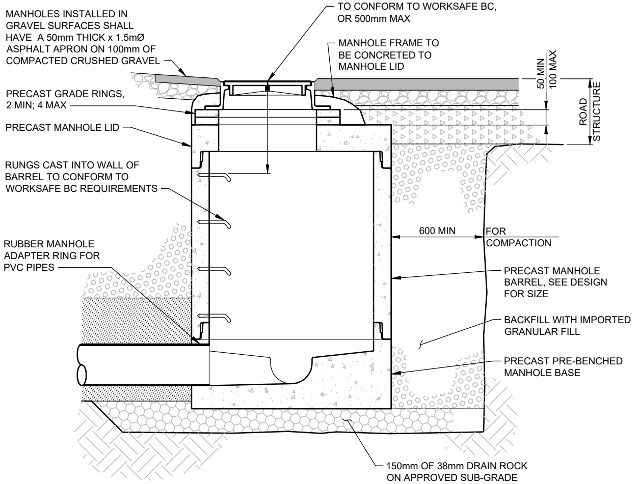
TYPICAL SECTION 1:25
