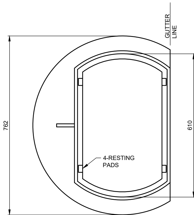
FRAME PLAN
