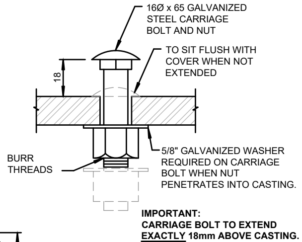
CARRIAGE BOLT DETAIL
