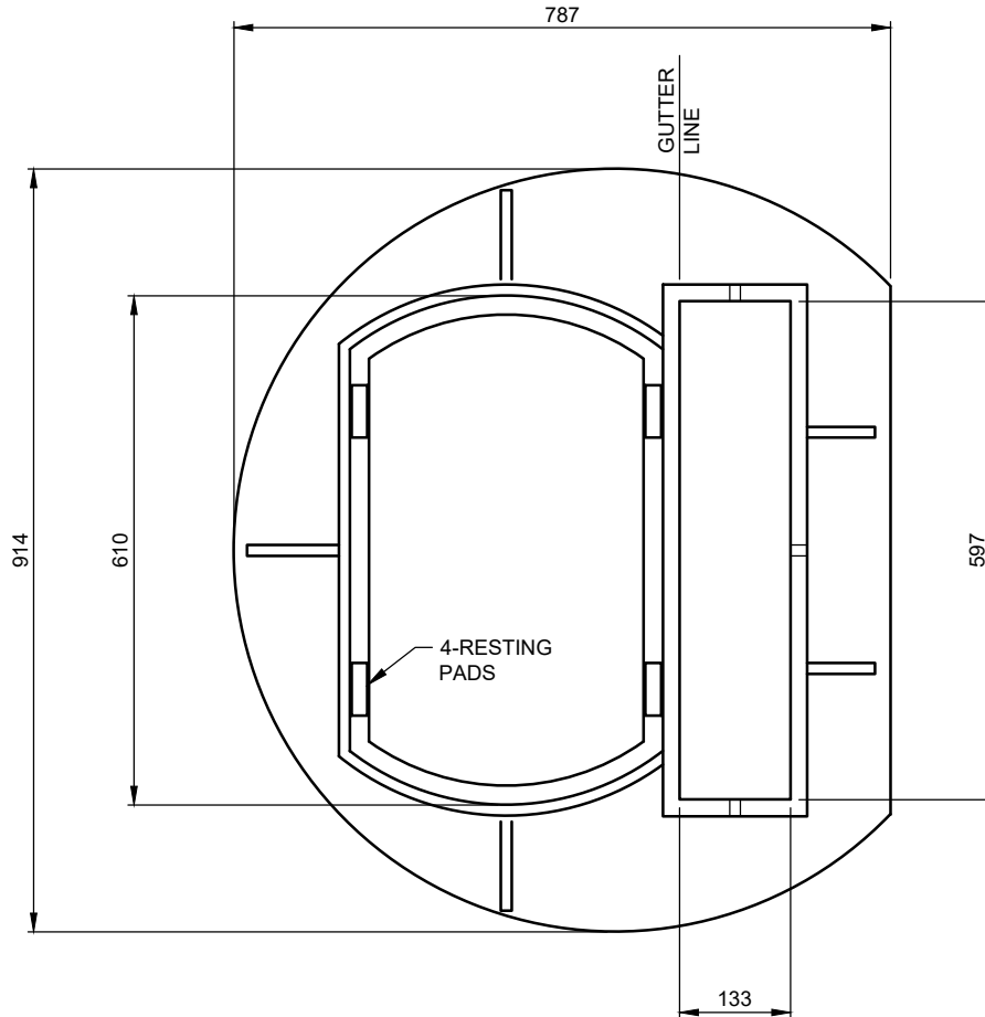
FRAME PLAN
