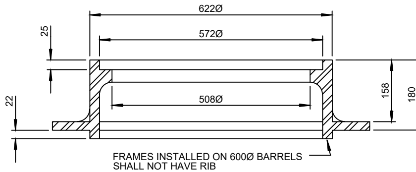
SECTION OF FRAME, RING AND COVER
