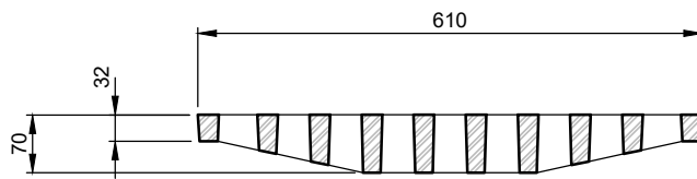
GRATE SECTION
