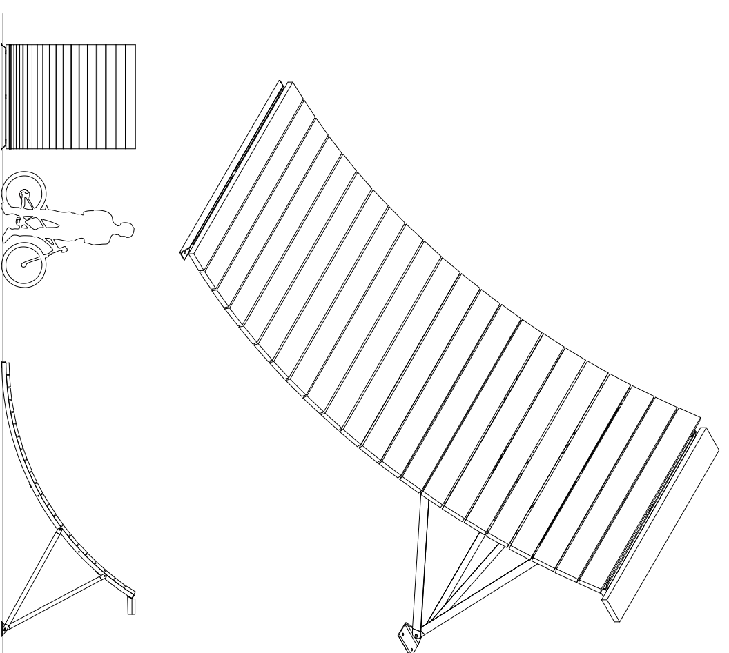
2 Launch Pad Feature (Large) by FlowForm Bike Ramps, Inc.
