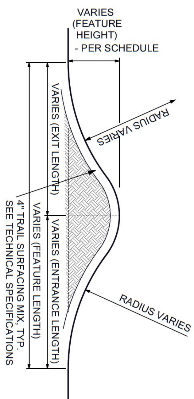
2 Roller - SECTION A
